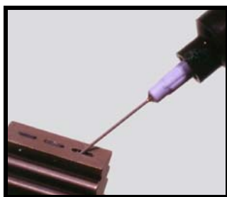
Figure 7. Core filling with a Burn-Off Masking Resin
