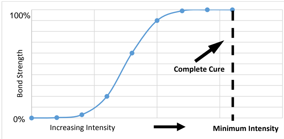
Figure 1. Curing Energy Profile (Exposure Time Held Constant)
