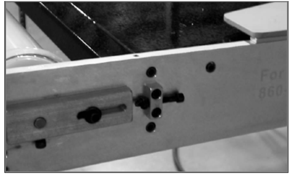
Figure 17. Adjustment Screws for Belt Tension and Alignment
