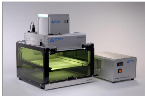
Dymax 5000 UV Curing Flood Lamp System Shown with Light Shield protective enclosure and ZIP™ shutter. Ideal for single component or batch curing processes requiring moderate intensity and a 12.7 cm x 12.7 cm cure area. CE Marked
