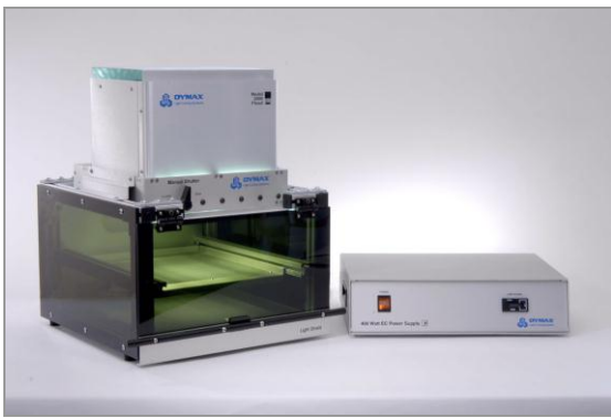
Dymax 2000 UV Curing Flood Lamp System Shown with Light Shield protective enclosure and manual shutter. Ideal for single component or batch curing processes requiring moderate intensity and a 8" x 8" (20.3 cm x 20.3 cm) cure area. CE Marked PC Series Flood Systems available for European production facilities.
