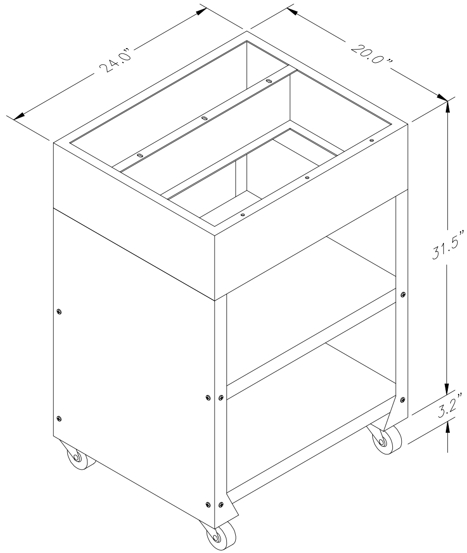
# 39215 CONVEYOR CART KIT OVERALL DIMS
